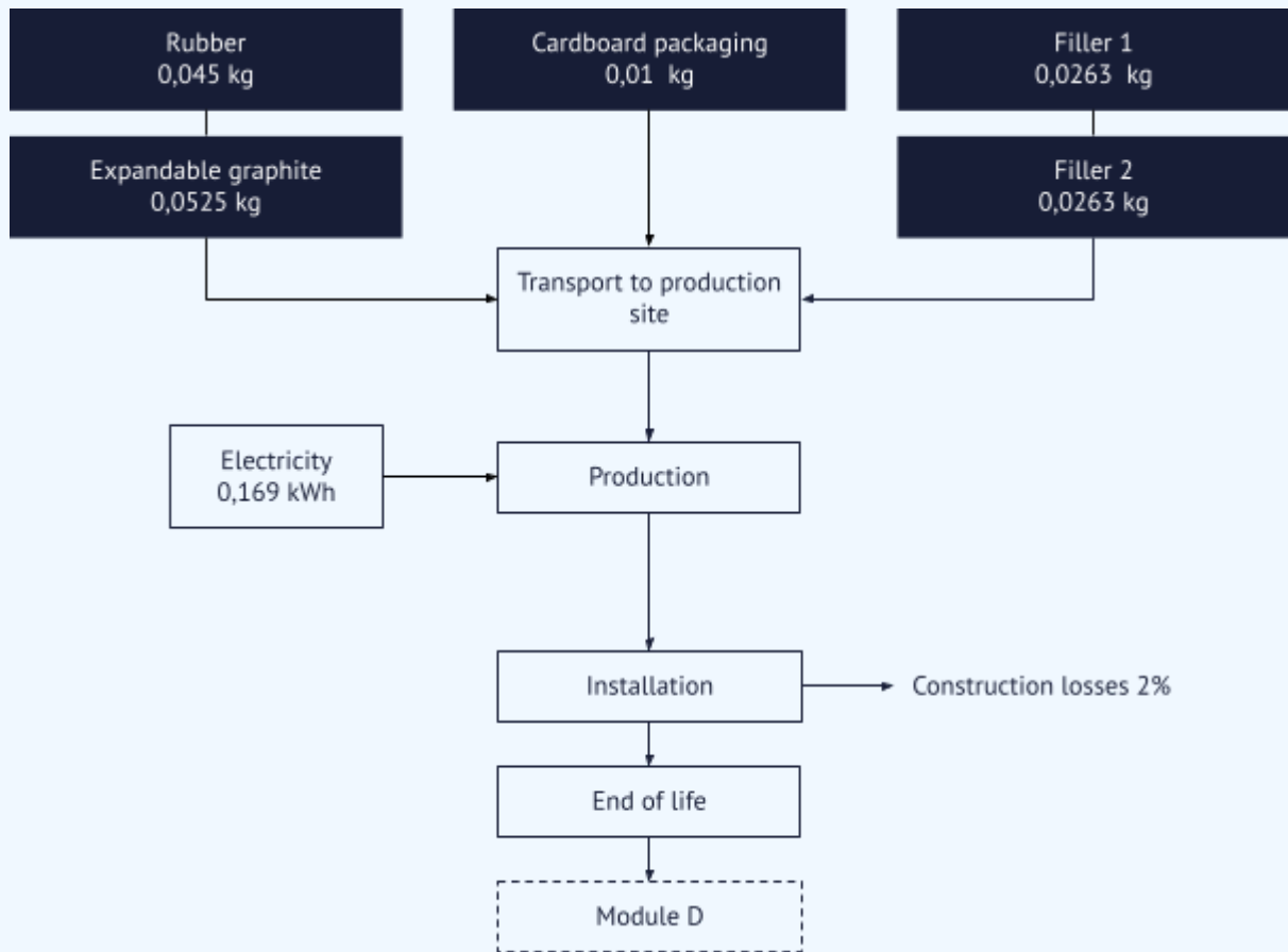
Figure 1. Flowchart of the product system under study, one metre of FIRESAFE FIRE Wrap.
